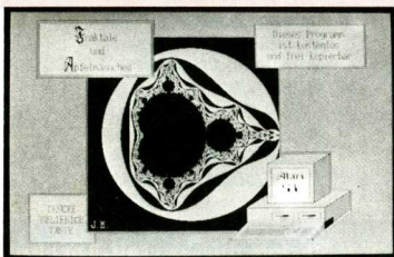
Fractals (PD23)
