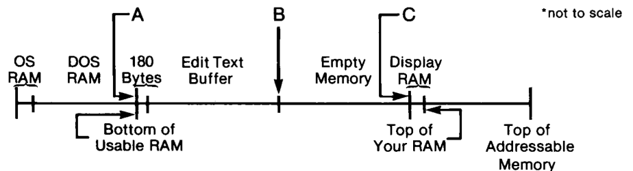
Figure 2. Memory map without use of LOMEN.
