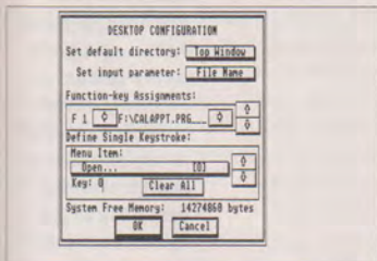
The look and feel of the Desktop can be altered from the Desktop Configuration, including the keystrokes for any of the menu options.
