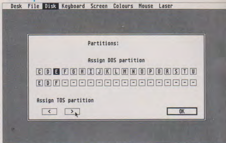
Mapping the hard drive partitions in the AT SPEED utility.
