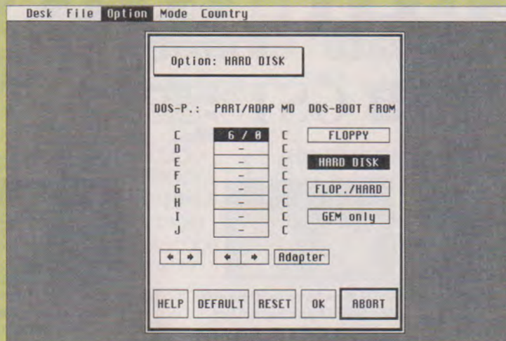
Mapping the hard disk partitions between TOS and DOS.
