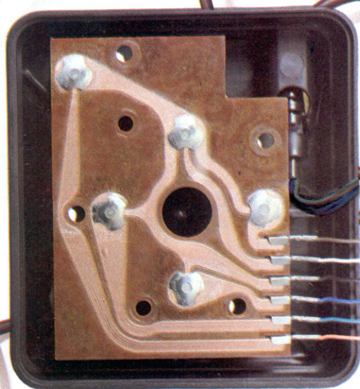
ORIGINAL WIRING
