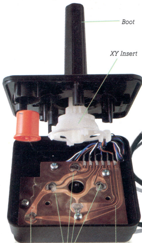
Boot XY Insert Directional Control Fire Control Printed Circuit Board
