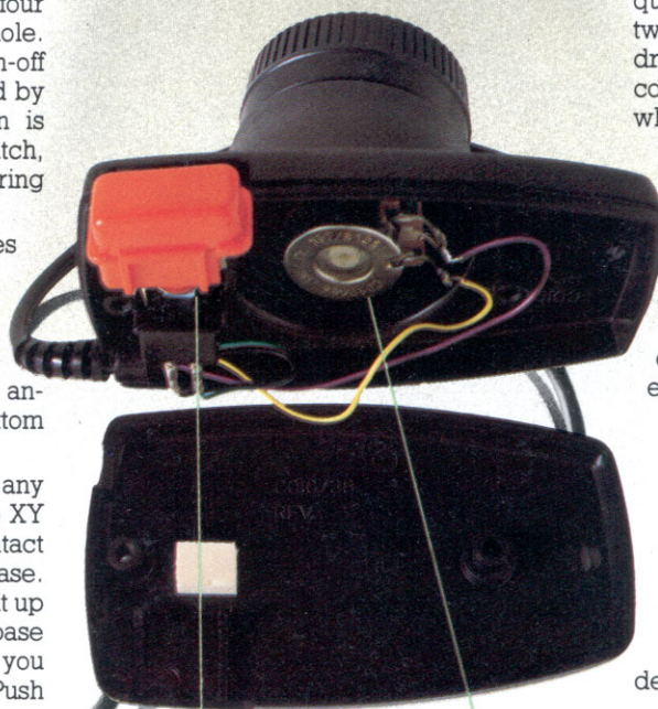
Fire Button Assembly Potentiometer
