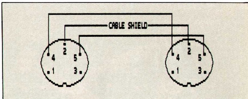
Figure 1. Schematic for standard MIDI cable. Shielded, twisted-pair cable should be used, with shield connected to pin 2 at either end.
