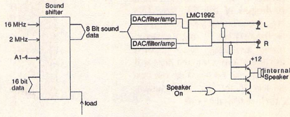
Figure 6 Sound Shifter
