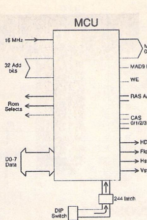
Figure 5 MCU
