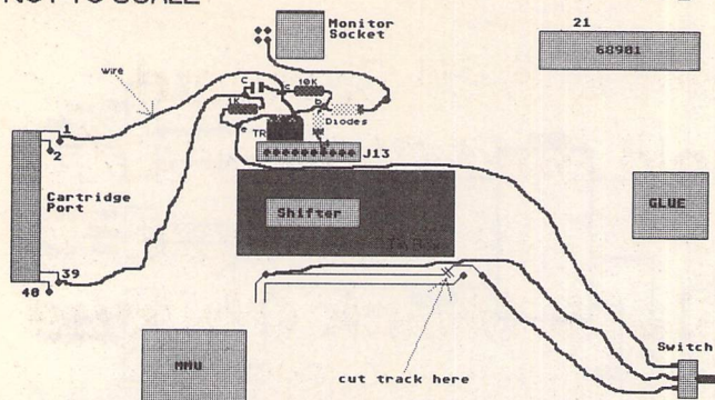
Overscan hardware mod for 520STFM by Jon Butler
