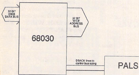
Figure 1 68030 busses
