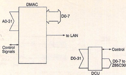
Figure 8 DMA
